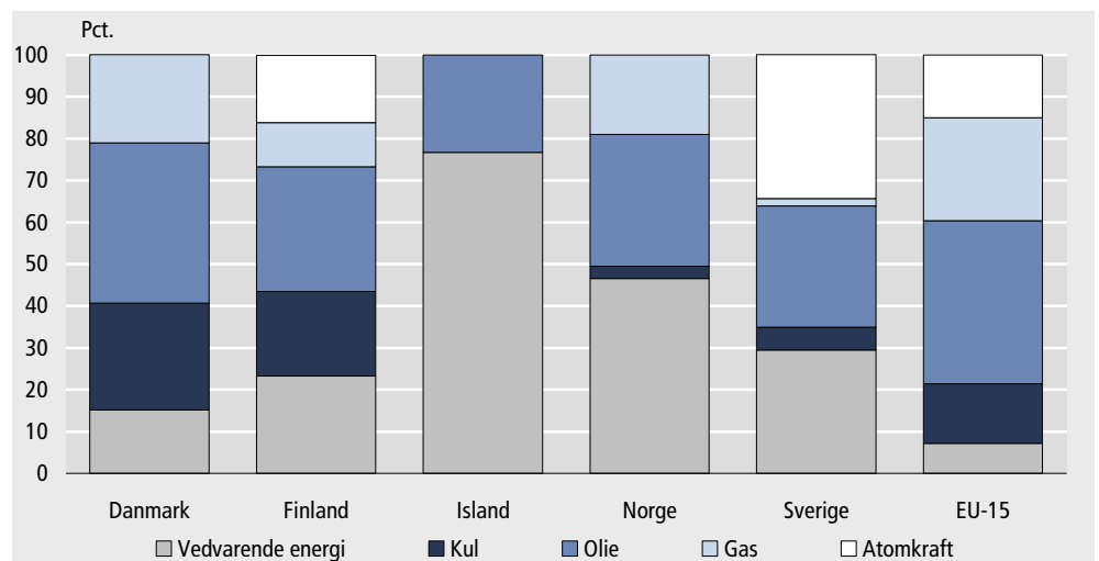
Figur 1. Energiforsyning. 2006
